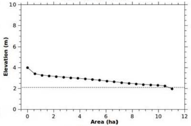
Kandoll Reference Hypsometric Curve
