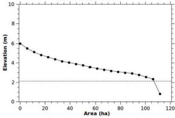
Kandoll Farm Hypsometric Curve
