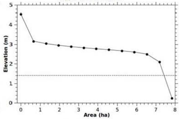
Vera Reference Hypsometric Curve
