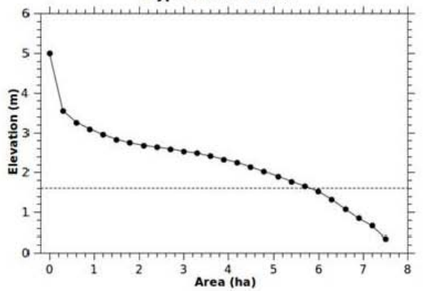
Vera Reference Hypsometric Curve
