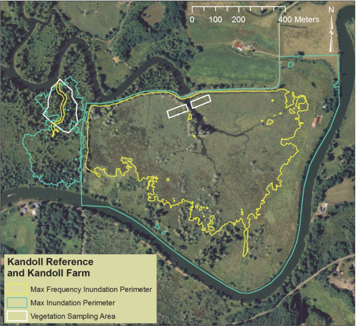
Inundation perimeters at the paired reference (east) and restoration sites (west). The inundation perimeters are model derived and represent the most frequently occurring water surface elevation (yellow) and the maximum water surface elevation (green).
