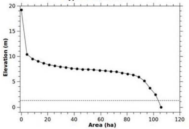
Vera Slough Hypsometric Curve
